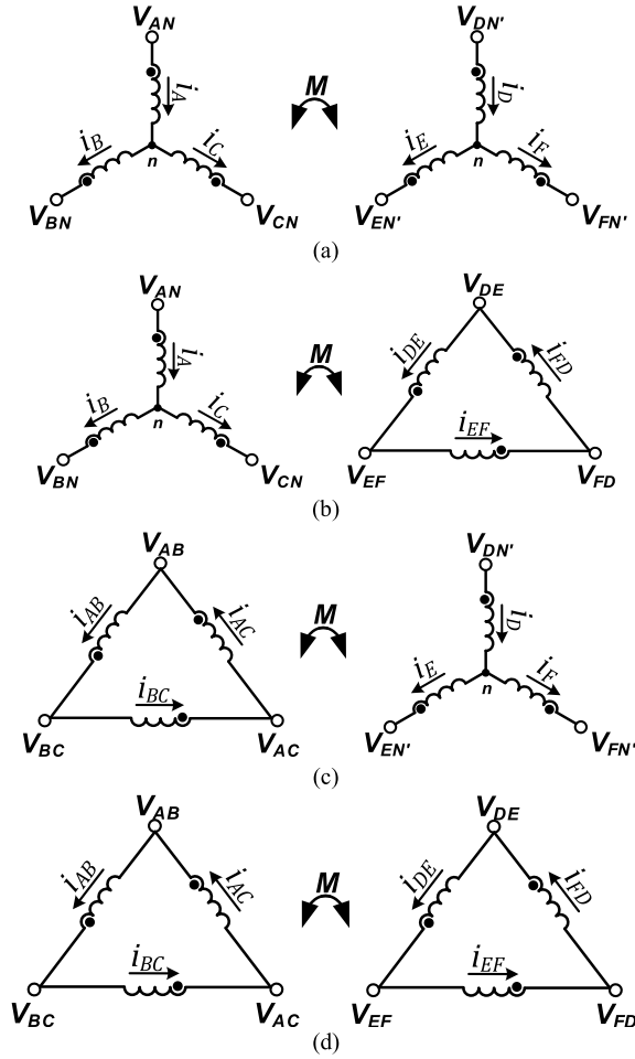
Fig. 5. Three-phase Tx and Rx coupler connection configurations; (a) Y/Y, (b) Y/Δ, (c) Δ/Y, and (d) Δ/Δ.
